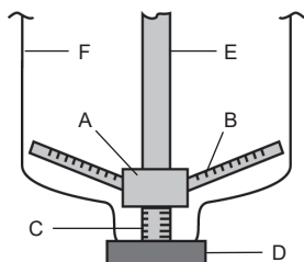
Z-style distributor shown mounted on blind flange.
